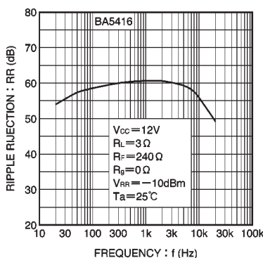
Fig. 26 Ripple rejection vs. frequency (BA5416)
