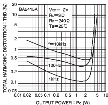
Fig. 14 Total harmonic distortion vs. output power (BA5415A)
