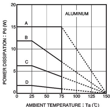
Fig. 11 Power dissipation curves (BA5416)
