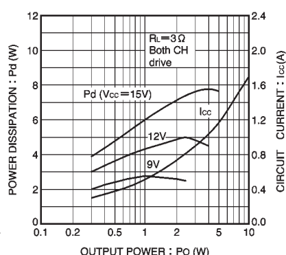
Fig. 30 Power dissipation and current vs. power supply voltage ( R_L = 3\Omega )
