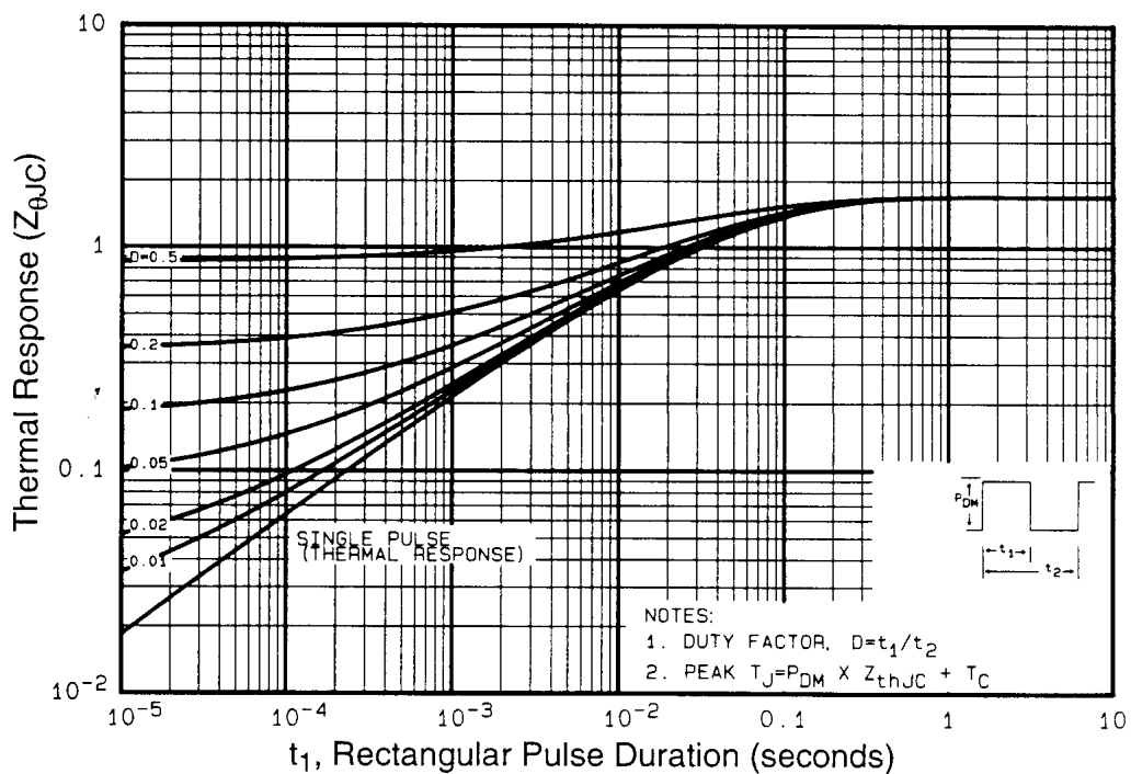
Fig 11. Maximum Effective Transient Thermal Impedance, Junction-to-Case
