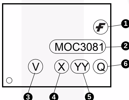
Figure 16. Top Mark
