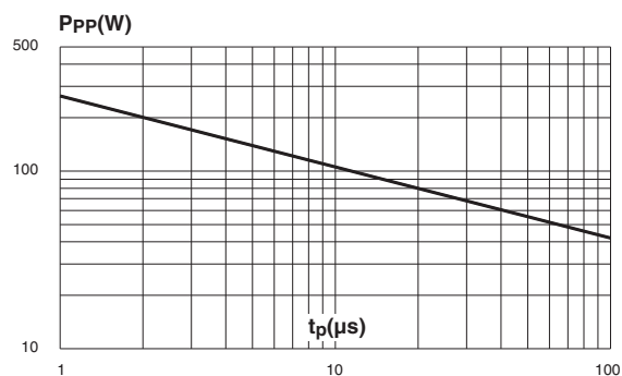
Figure 3: Peak pulse power versus exponential pulse duration
