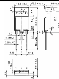
TO-3PM
