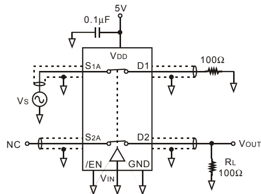
Fig.8 Crosstalk
