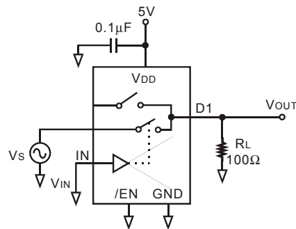
Fig.7 Bandwidth Testing
