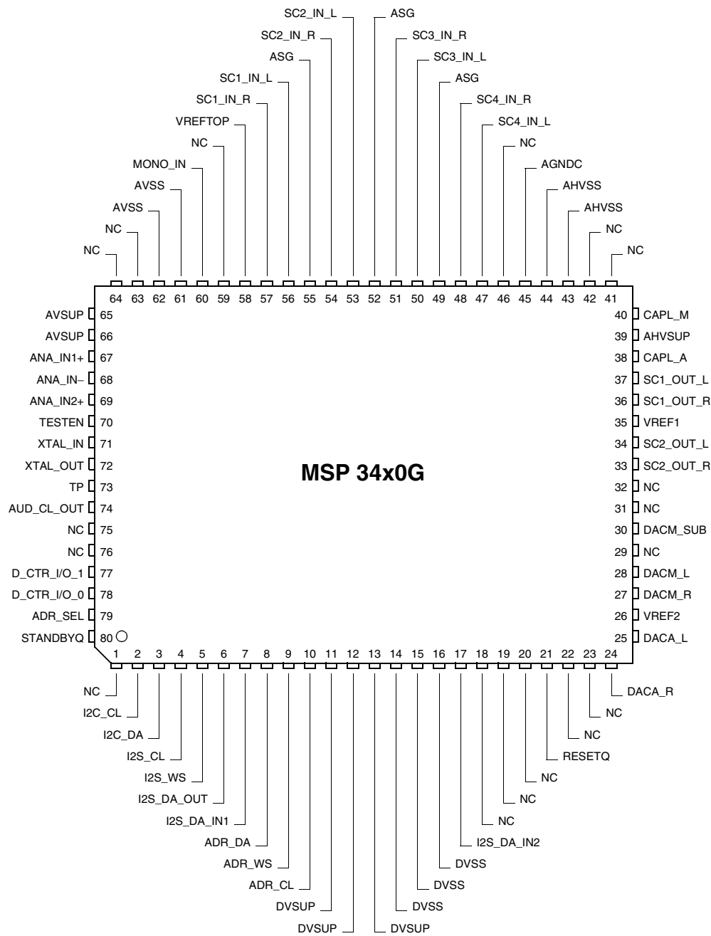
Fig. 4–8: PMQFP80-11 package
