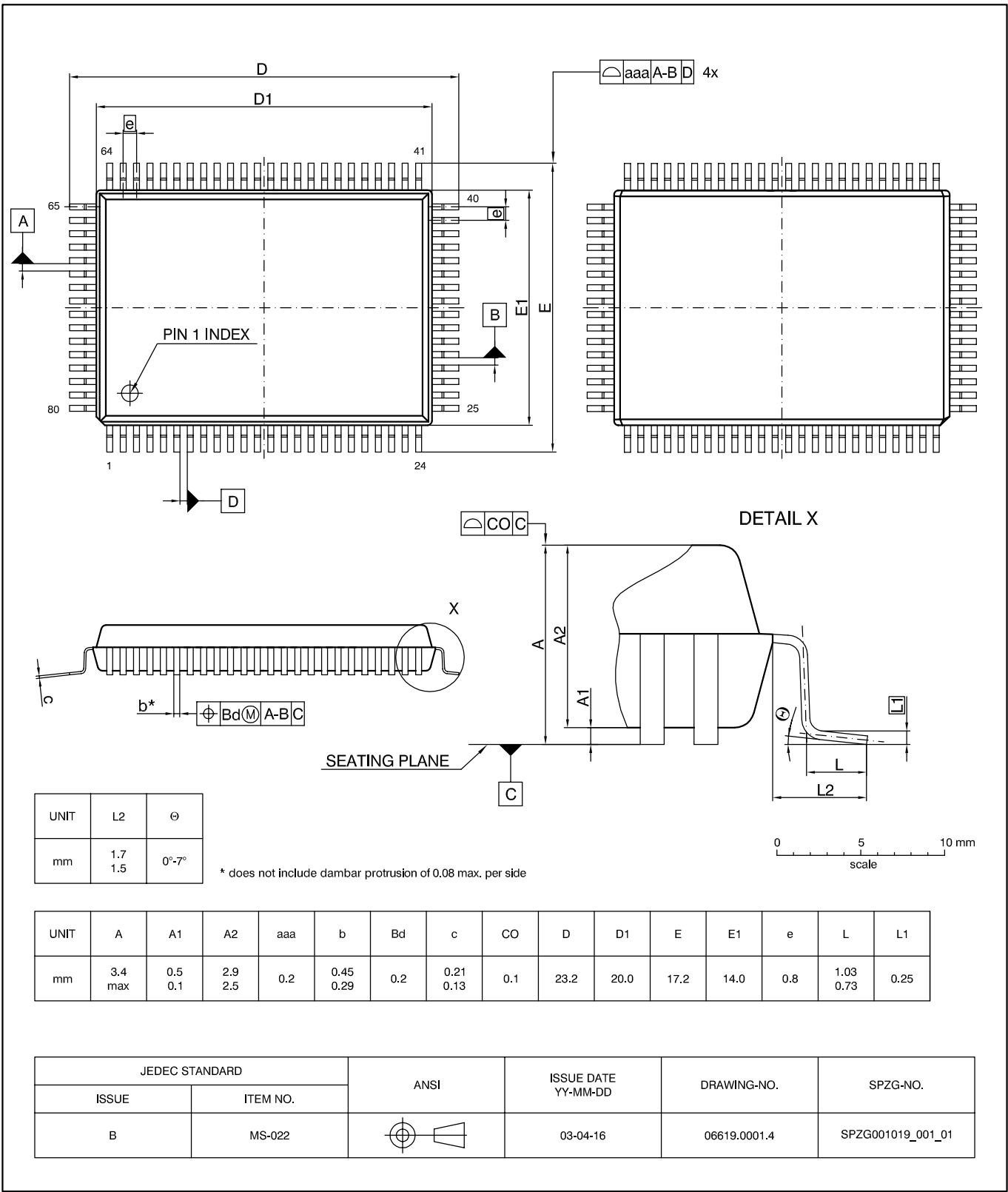
Fig. 4-4: PMQFP80-11: Plastic Metric Quad Flat Package, 80 leads, 14 \times 20 \times 2.7 \text{ mm}^3 , high standoff Ordering code: QA Weight approximately 1.68 g
