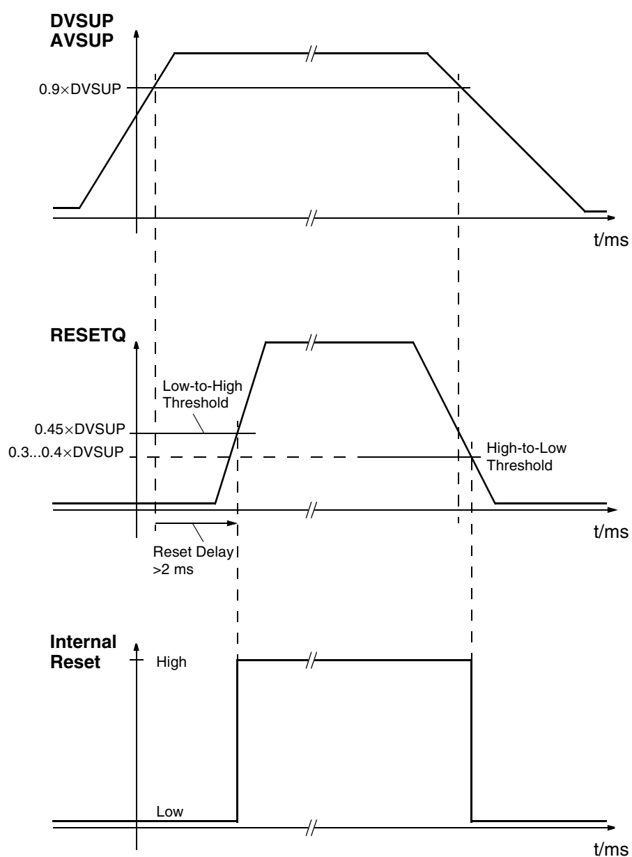
Fig. 4-25: Power-up sequence
