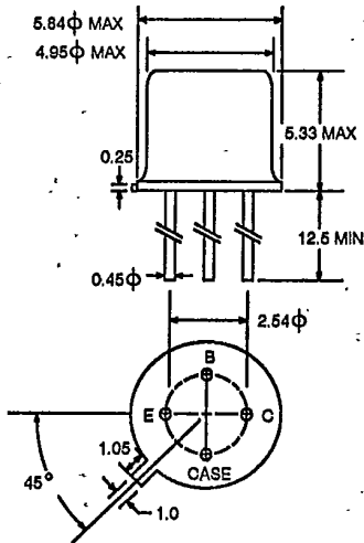
OUTLINE 35 (MICRO-X)
