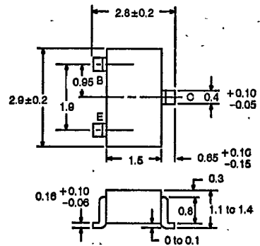
OUTLINE 33 (SOT-23)
