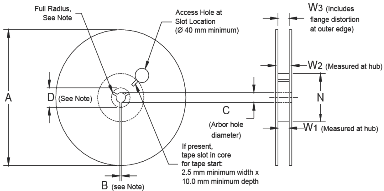
Figure 6 – Reel Dimensions
