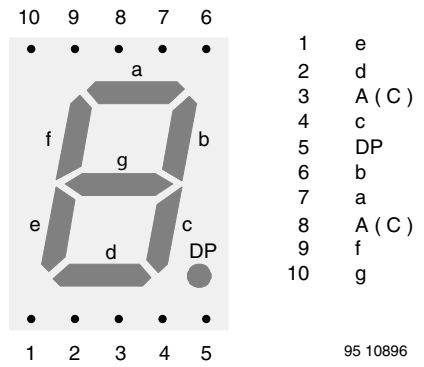
Fig. 7 - TDSR1350, TDSR1360
