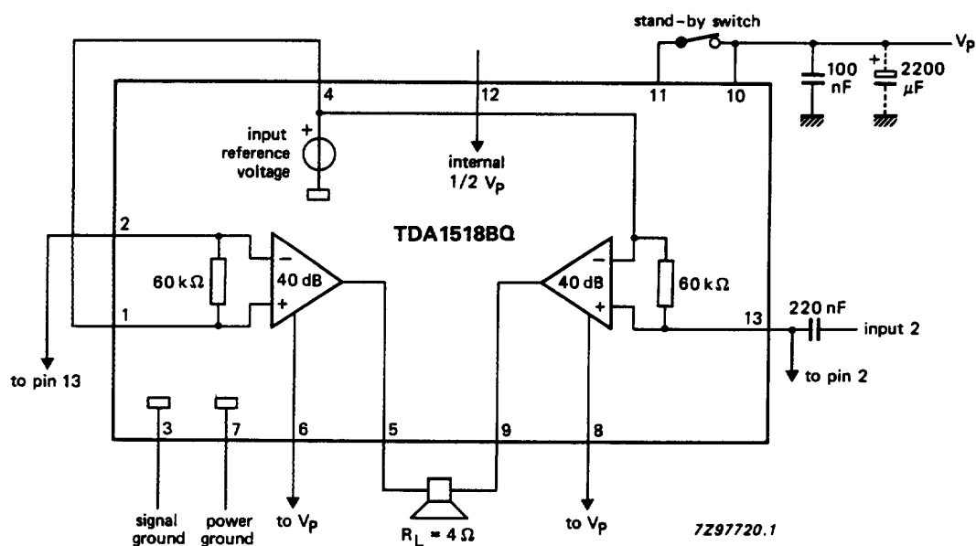
Fig.4 BTL application circuit diagram (without bootstrapping).
