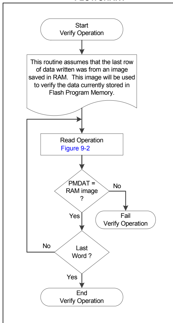
FIGURE 9-8: FLASH PROGRAM MEMORY VERIFY FLOWCHART
