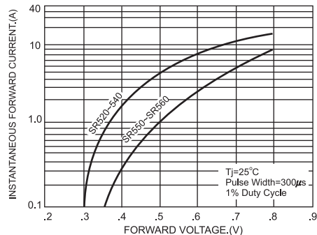
FIG.4-TYPICAL FORWARD CHARACTERISTICS
