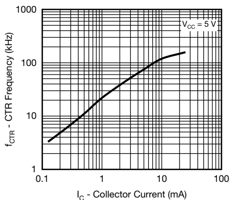
Fig. 12 - CTR Frequency vs. Collector Current
