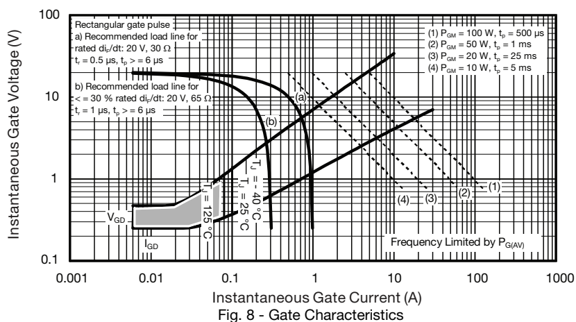
Fig. 8 - Gate Characteristics
