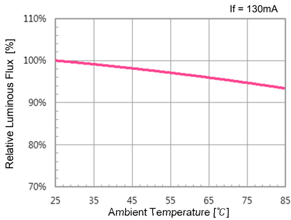
▪ Luminous Flux vs. Temp.
