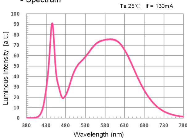
▪ Radiation Characteristics
