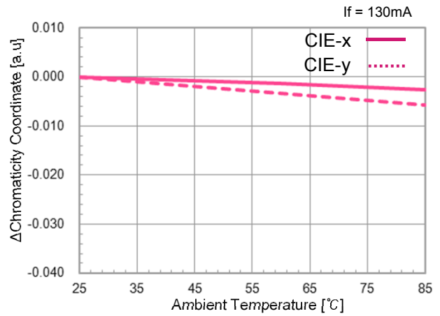
▪ CIE vs. Temp.
