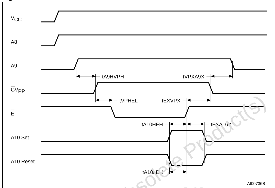
Figure 7. MARGIN MODE AC Waveforms
