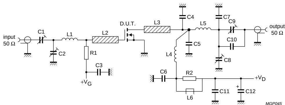
Fig.14 Test circuit for class-AB operation.
