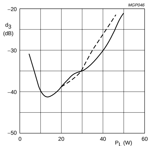
Class-AB operation; V_{DS} = 28\text{ V} ; I_{DQ} = 0.25\text{ A} ; R_{th\text{ mb-h}} = 0.3\text{ K/W} ; f = 28\text{ MHz} . solid line: T_h = 25^\circ\text{C} . dotted line: T_h = 70^\circ\text{C} .
