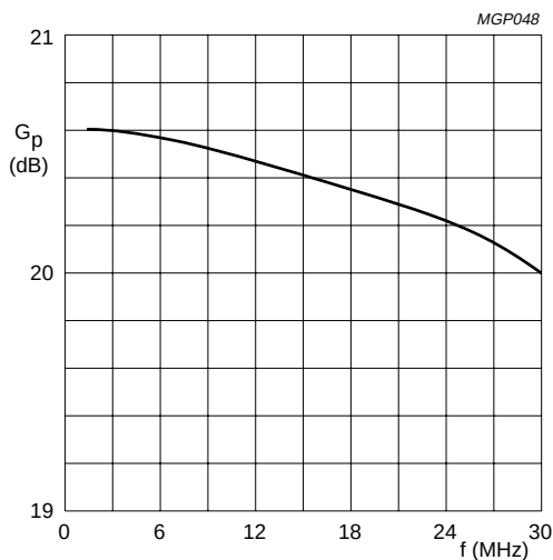
Class-AB operation; V_{DS} = 28\text{ V} ; I_{DQ} = 0.25\text{ A} ; P_L = 30\text{ W} ; T_h = 25^\circ\text{C} ; R_{th\text{ mb-h}} = 0.3\text{ K/W} ; R_1 = 34\ \Omega ; Z_L = 8.9 + j1\ \Omega .
