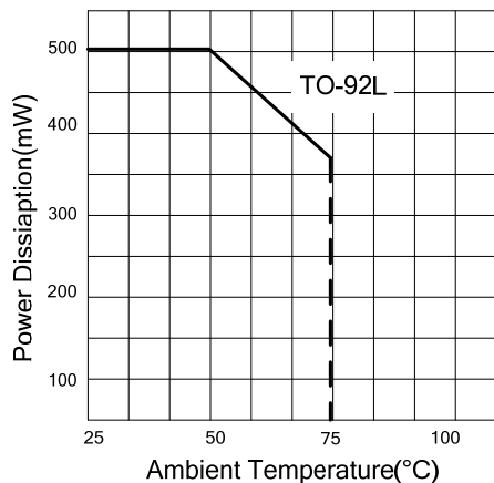
Fig.1 Ambient Temperature vs. Power Dissipation
