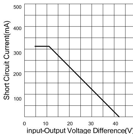
Fig.6 Short Circuit Output Current ( T_J=25^\circ C )
