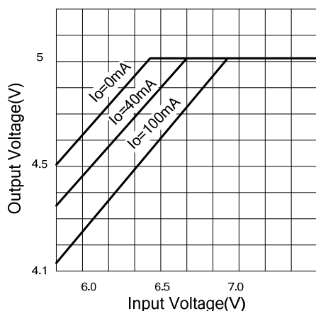
Fig.5 UTC78L05M Dropout Characteristics ( T_J=25^\circ C )
