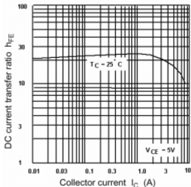
Fig.3 DC current Gain
