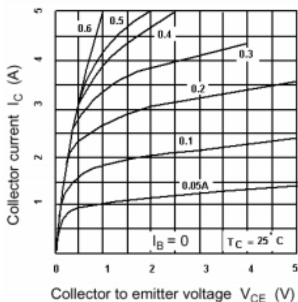
Fig.4 Static Characteristic
