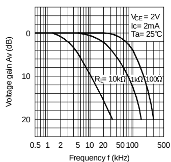
Fig.11 Frequency Response
