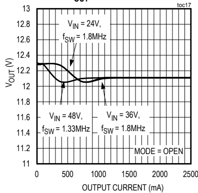
LOAD REGULATION V OUT = 12V, PFM MODE
