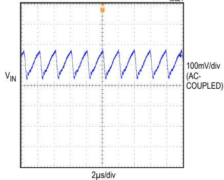
INPUT VOLTAGE RIPPLE V IN = 24V, V OUT = 3.3V, I OUT = 2.5A, MODE = SGND
