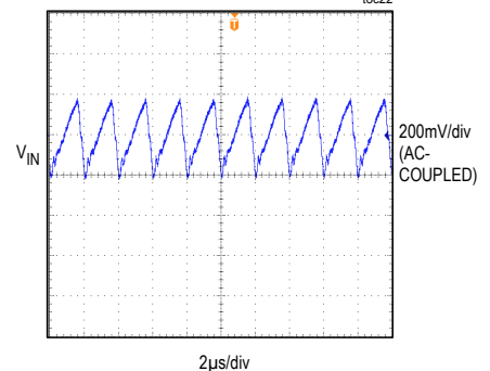
INPUT VOLTAGE RIPPLE V IN = 24V, V OUT = 5V, I OUT = 2.5A, MODE = SGND
