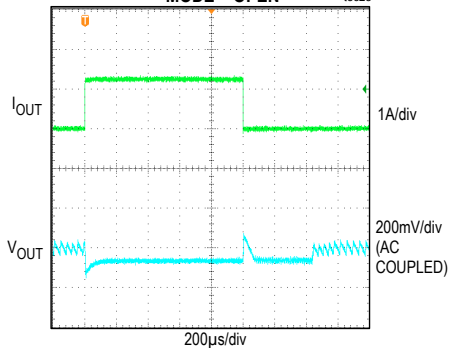
LOAD CURRENT TRANSIENT RESPONSE V IN = 24V, V OUT = 3.3V, I OUT = 0.05A - 1.25A, MODE = OPEN
