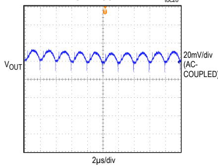
OUTPUT VOLTAGE RIPPLE V IN = 24V, V OUT = 5V, I OUT = 2.5A, MODE = SGND
