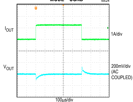
LOAD CURRENT TRANSIENT RESPONSE V IN = 24V, V OUT = 3.3V, I OUT = 0.05A - 1.25A, MODE = SGND
