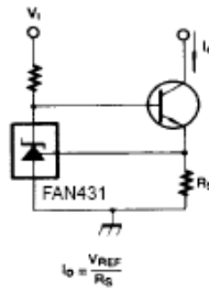
Figure 17. Constant-Current Sink
