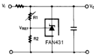
Figure 13. Shunt Regulator
