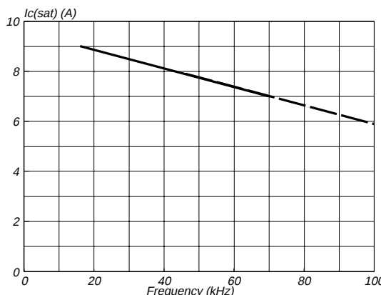
Fig. 12. I_{Csat} during normal running vs. frequency of operation for optimum performance
