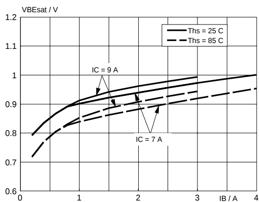
Fig. 8. Typical base-emitter saturation voltage.
