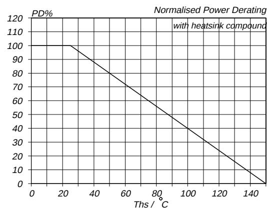
Fig. 10. Normalised power dissipation. PD\% = 100 \cdot P_D / P_{D 25^\circ C}
