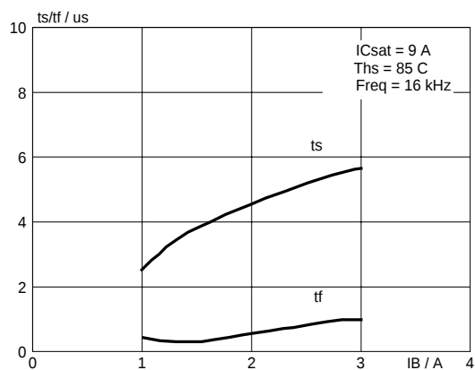
Fig. 9. Typical collector storage and fall time. I_{Csat} = 9A ; T_j = 85^\circ C ; f = 16kHz
