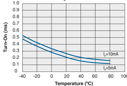
Typical Turn-On vs. Temperature ( I_L=50mA )
