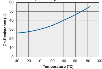
Typical On-Resistance vs. Temperature ( I_F=0mA, I_L=Max\ Rated )
