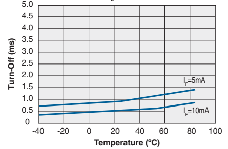
Typical Turn-Off vs. Temperature ( I_L=50mA )
