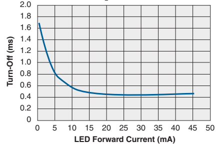
Typical Turn-Off vs. LED Forward Current ( I_L=100mA )
