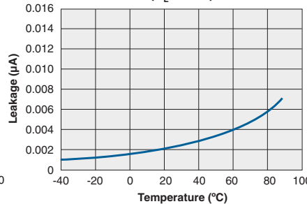
Typical Leakage vs. Temperature Measured Across Pins 3&4 ( V_L=350V )
